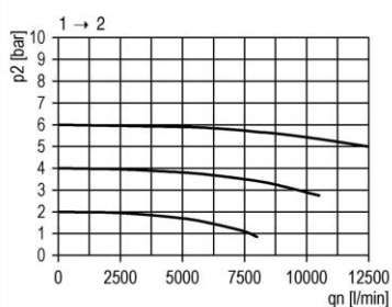
flow characteristic
